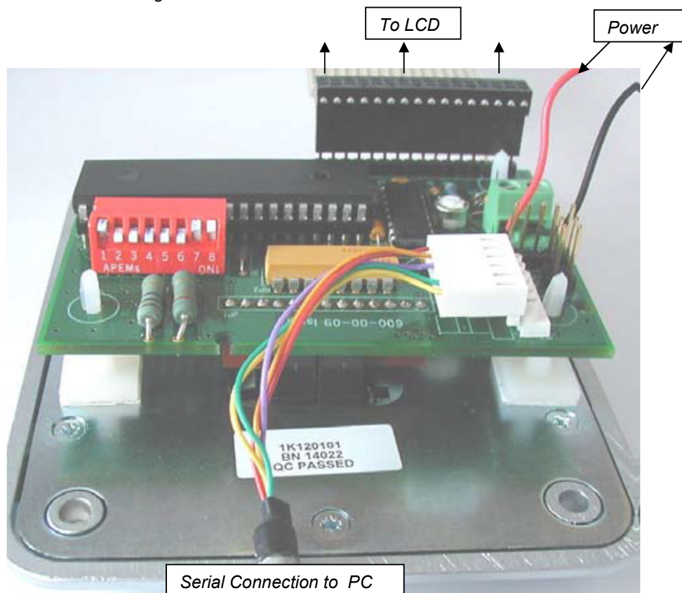
Typical picture showing encoder mounted directly to pinpad.
